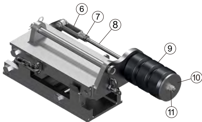
LH Wing Trip Assembly
