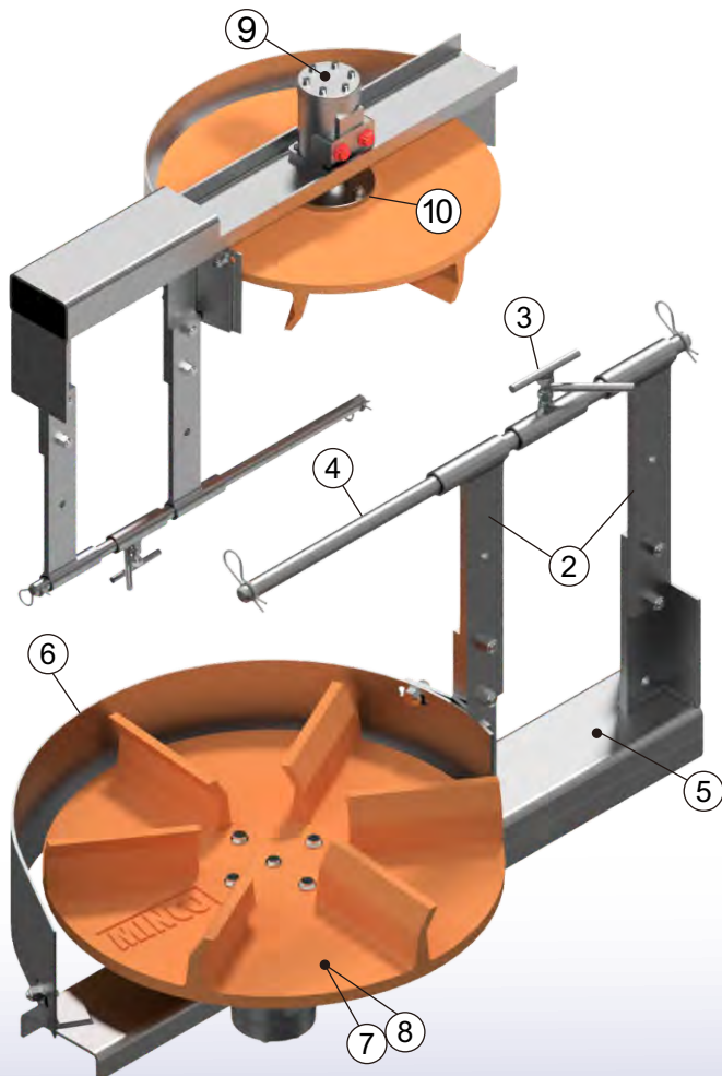
Heavy Duty Ice Chopper
