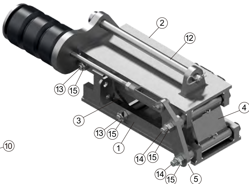
RH Wing Trip Assembly
